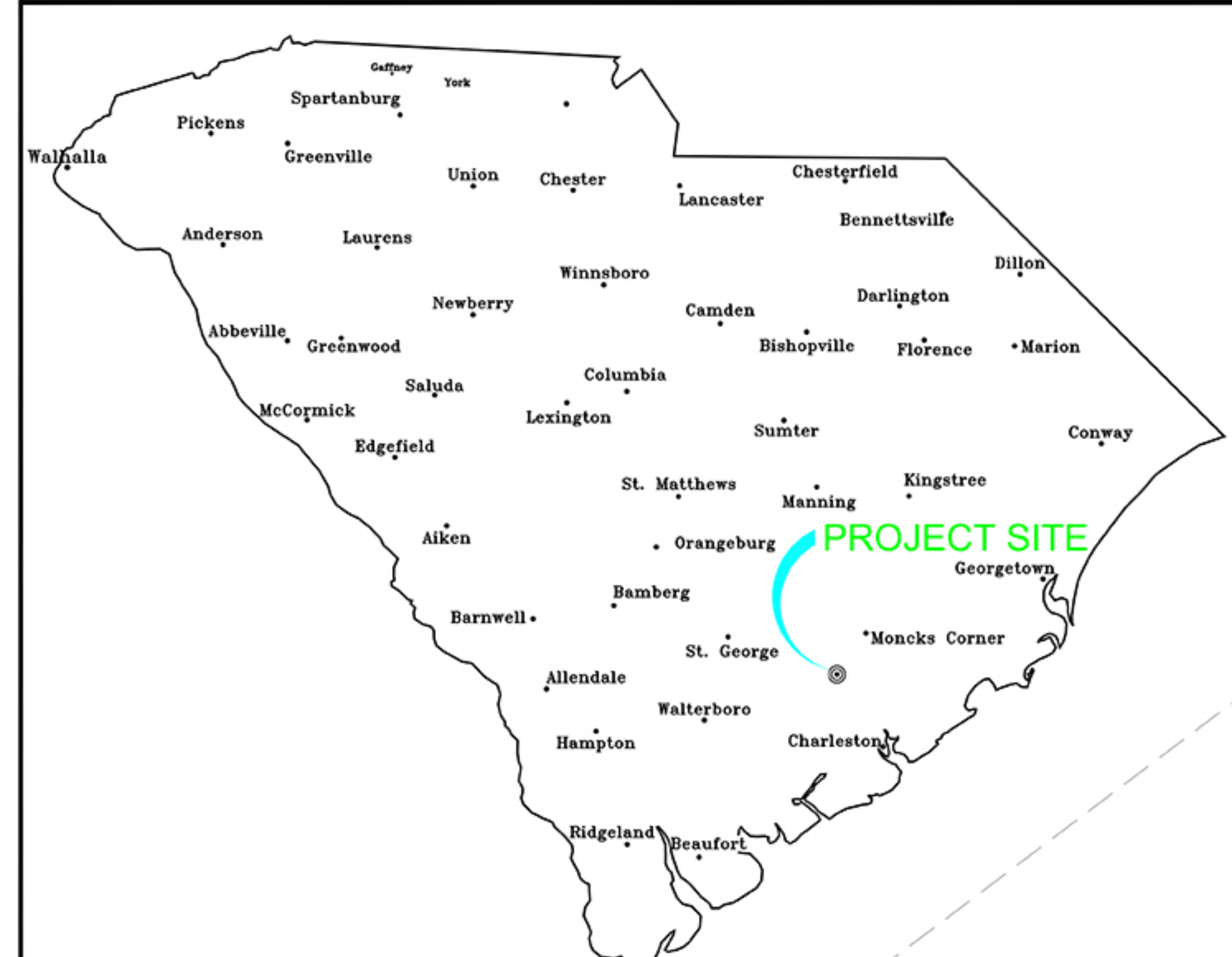
VICINITY MAP
